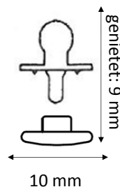
LOXX® lower part for riveting
